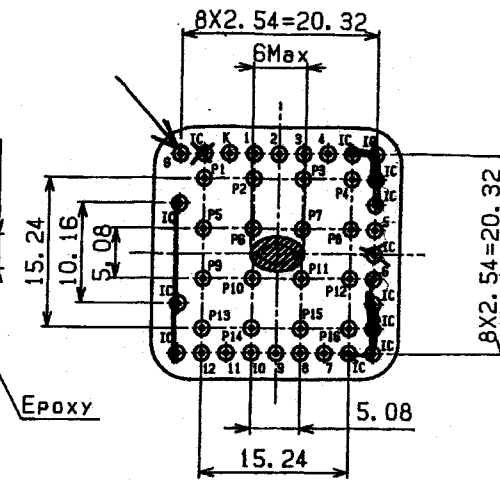
Bottom View IC: Internal Connection (Do not use)
